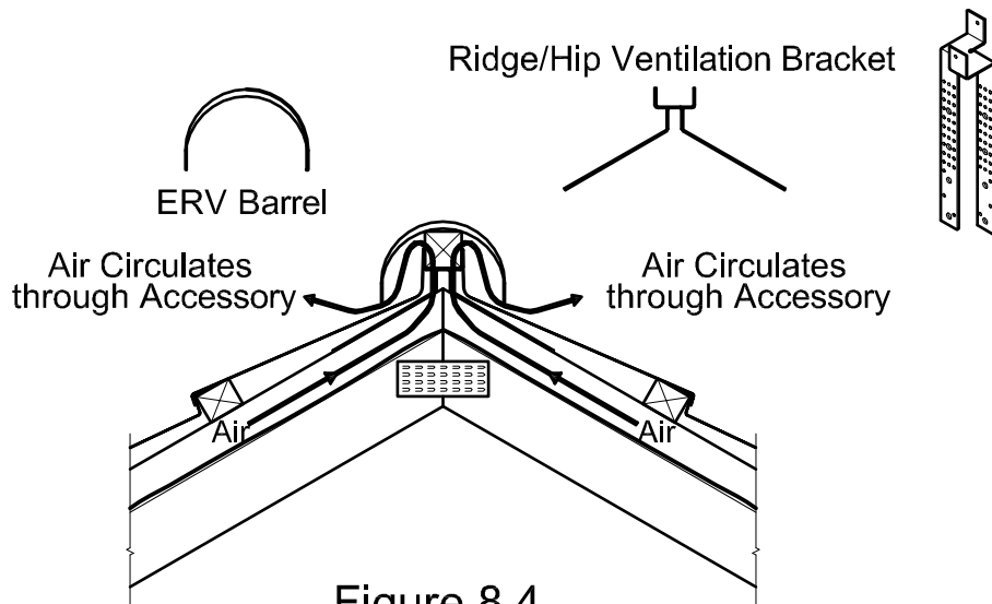
Figure 8.4 ERV Barrel -Ventilated
