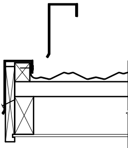
Figure 9.1 Box Barge
