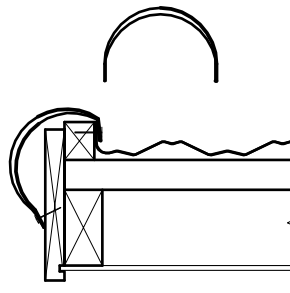
Figure 9.2 Barrel
