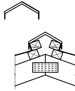
Figure 8.3 Angle Trim
