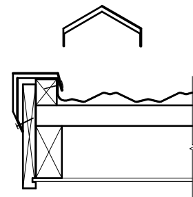
Figure 9.3 Angle Trim
