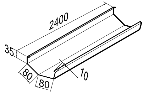
Figure 7.10 Valley
