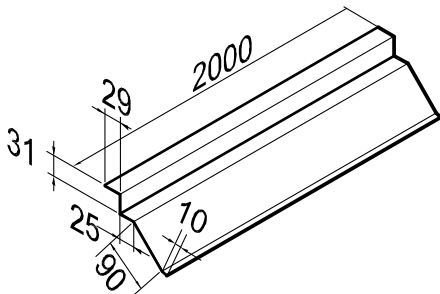
Figure 7.13 Eaves Starter Flashing
