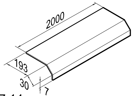
Figure 7.14 Top Course
