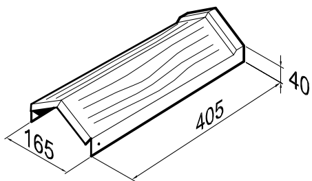
Figure 7.7 Angle Trim
