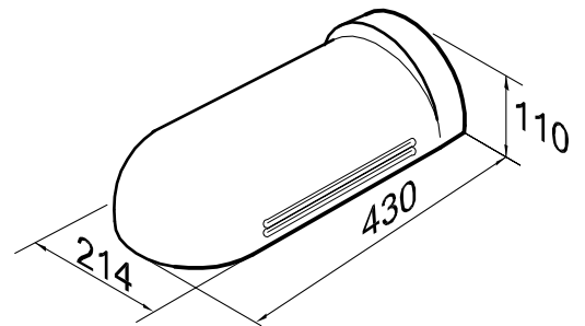
Figure 7.6 ERV Barrel Moulded End
