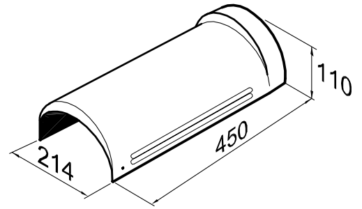
Figure 7.2 ERV Barrel
