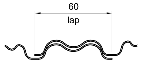
Figure 3.2 Nailing Detail
