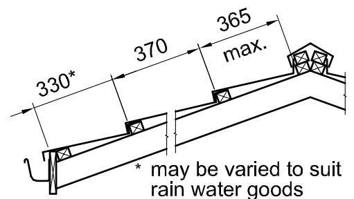
Figure 3.5 Batten Layout
