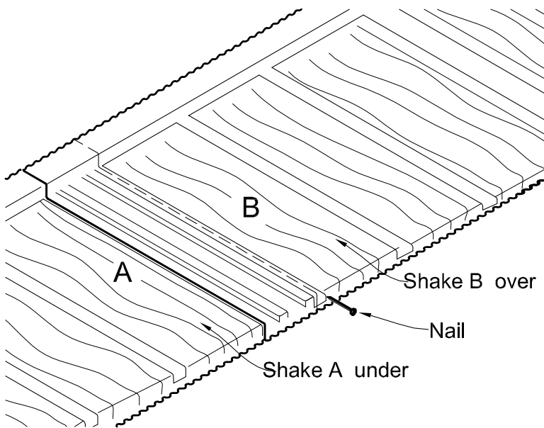
Figure 3.3 Overlap Detail
