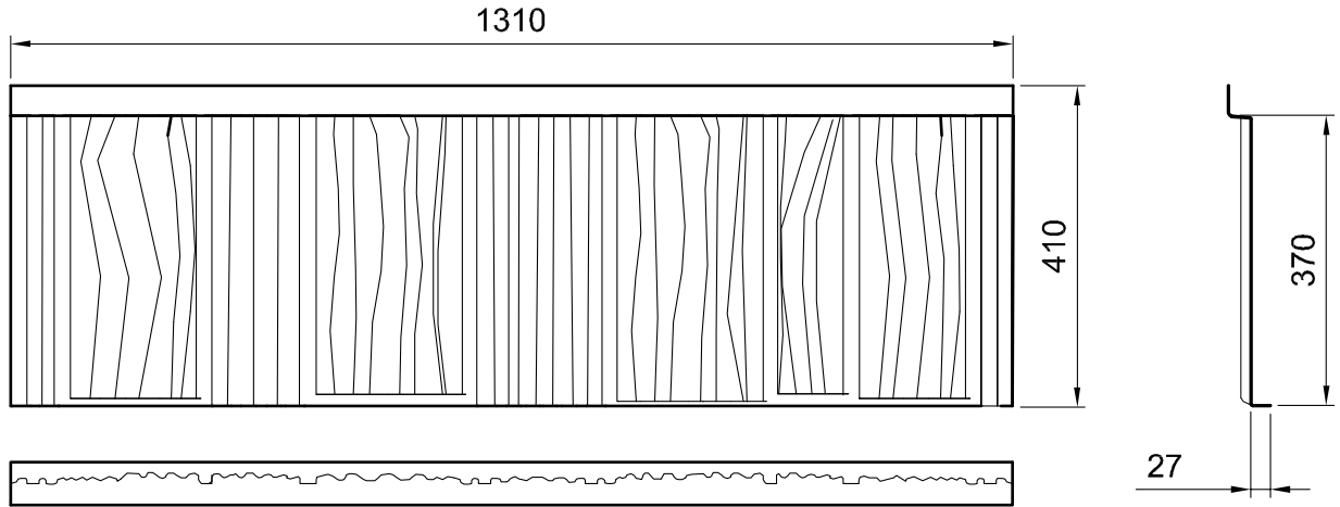
Figure 3.1 Shake Dimensions
