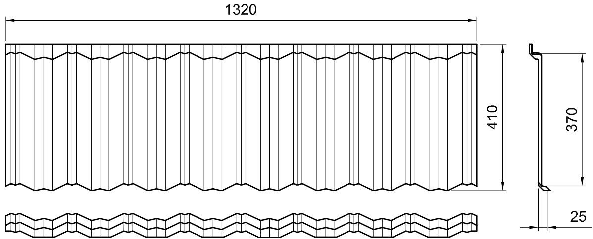
Figure 1.1 Tile Dimensions
