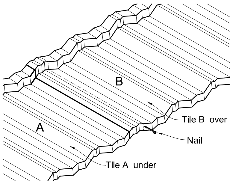
Figure 1.3 Overlap Detail
