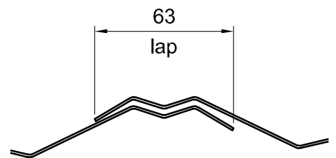
Figure 1.4 Lap Detail
