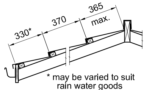
Figure 1.5 Batten Layout
